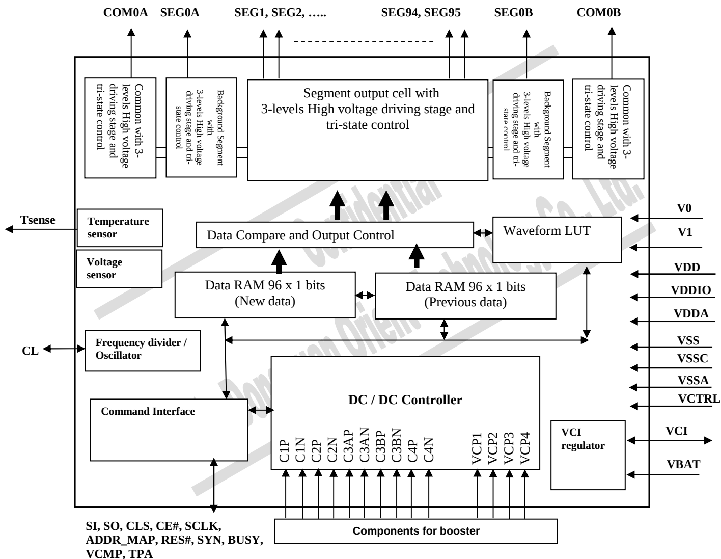
Figure 4-2: SSD1623 DC/DC Block Diagram
